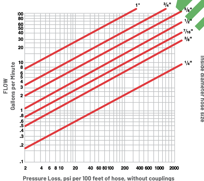
Pressure Loss at Various Rates of Flow of Water Through Hose*
